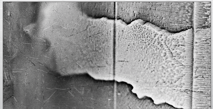
Picture: visualization of grain-oriented electrical steel
